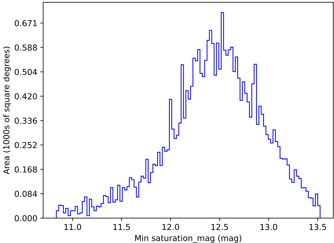
too_elab_r32_d3_gz_v3.4_10yrs All sky i band: Min saturation_mag
