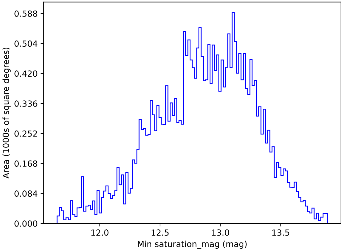
too_elab_r32_d3_gz_v3.4_10yrs All sky g band: Min saturation_mag
