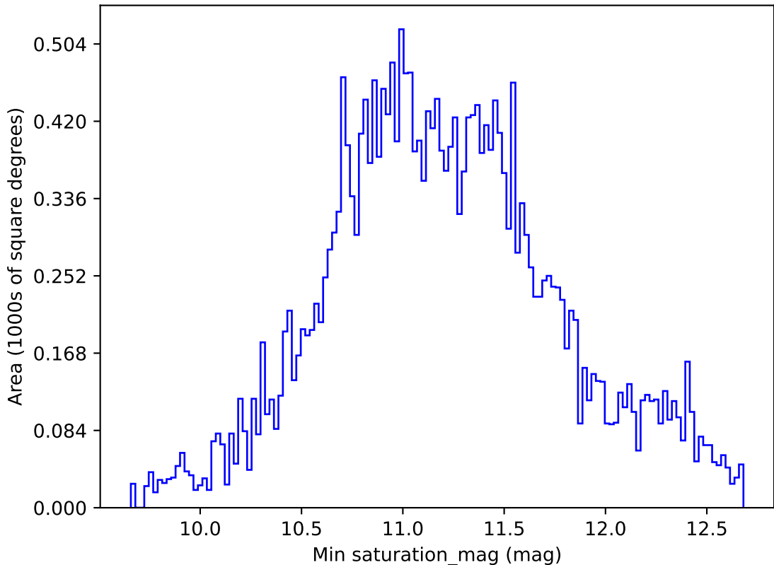
too_elab_r32_d3_gz_v3.4_10yrs All sky all bands: Min saturation_mag
