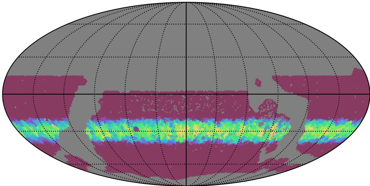
too_elab_r32_d3_gz_v3.4_10yrs WFD r band: Min normairmass
