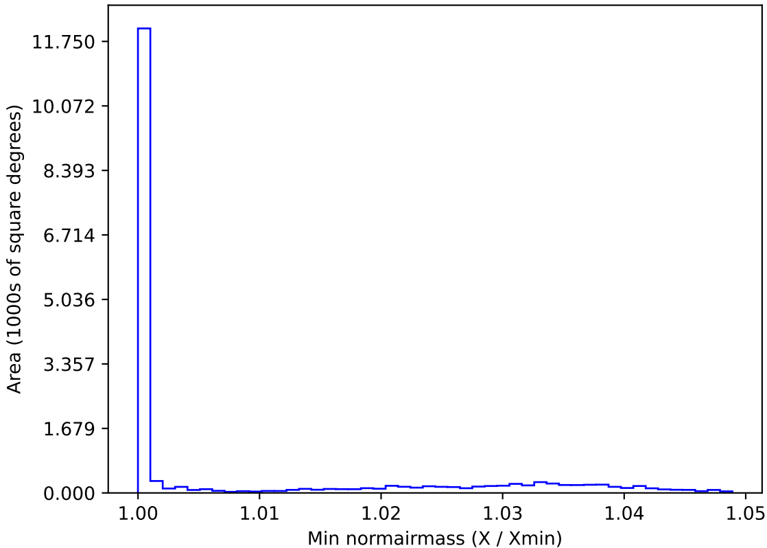
too_elab_r32_d3_gz_v3.4_10yrs WFD g band: Min normairmass
