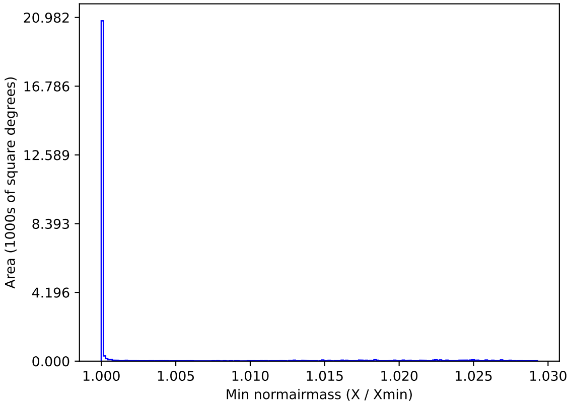
too_elab_r32_d3_gz_v3.4_10yrs All sky all bands: Min normairmass
