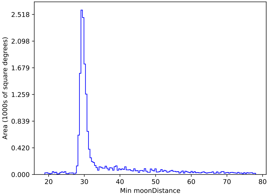
too_elab_r32_d3_gz_v3.4_10yrs WFD z band: Min moonDistance
