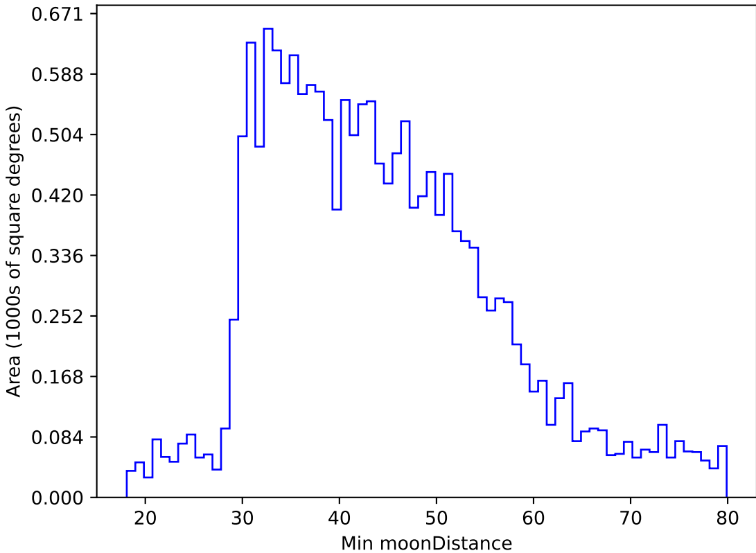
too_elab_r32_d3_gz_v3.4_10yrs WFD g band: Min moonDistance
