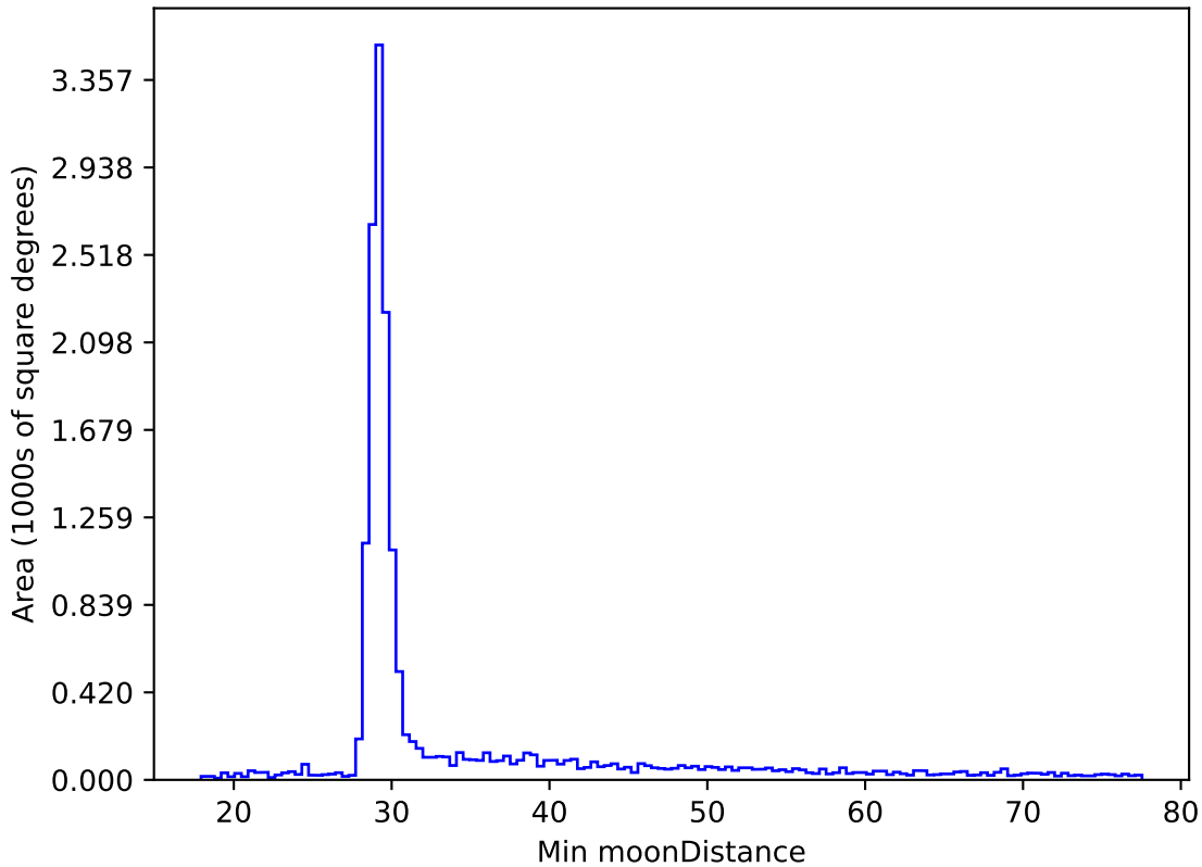
too_elab_r32_d3_gz_v3.4_10yrs WFD all bands: Min moonDistance
