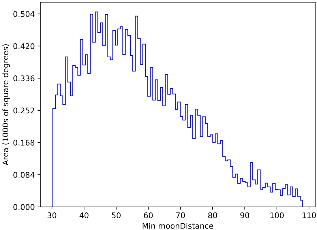
too_elab_r32_d3_gz_v3.4_10yrs All sky u band: Min moonDistance
