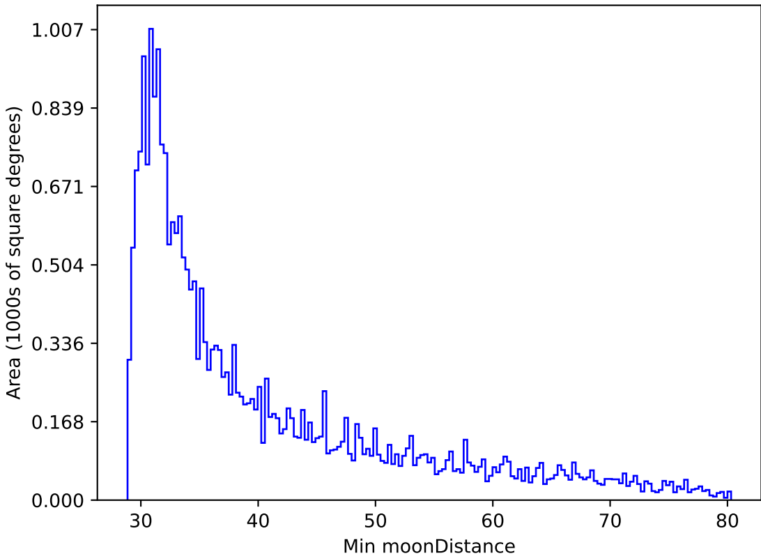
too_elab_r32_d3_gz_v3.4_10yrs All sky r band: Min moonDistance
