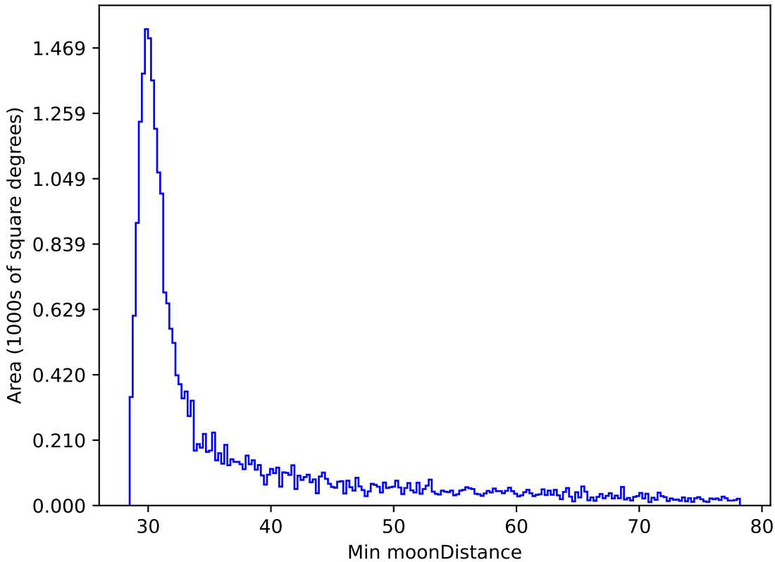
too_elab_r32_d3_gz_v3.4_10yrs All sky i band: Min moonDistance
