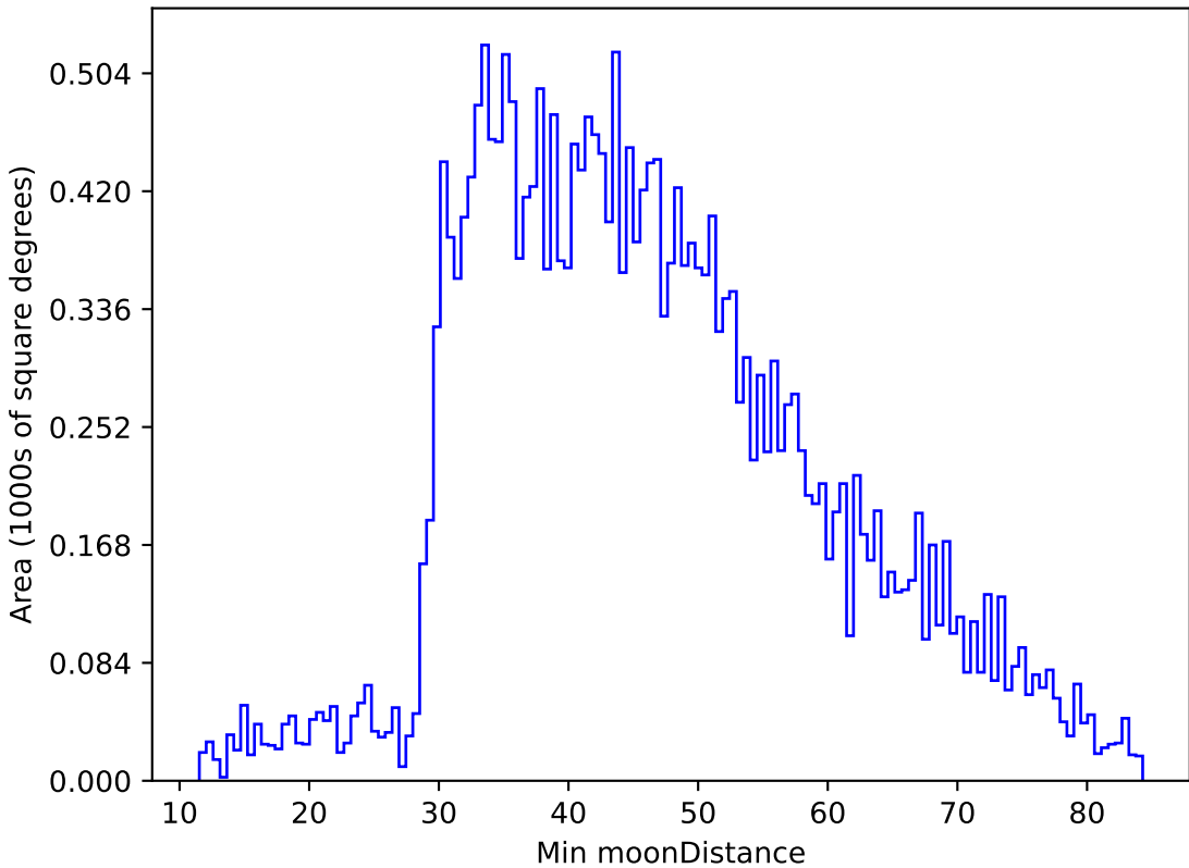
too_elab_r32_d3_gz_v3.4_10yrs All sky g band: Min moonDistance
