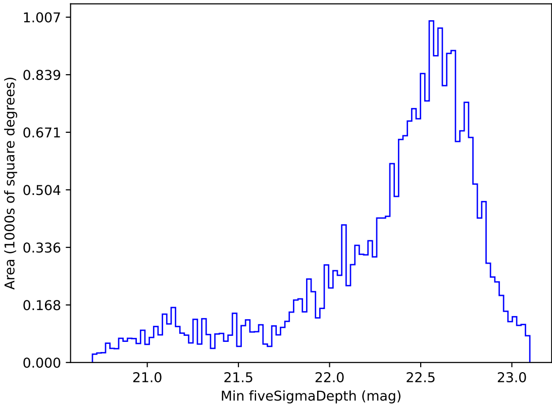
too_elab_r32_d3_gz_v3.4_10yrs Yr 1 z band: Min fiveSigmaDepth
