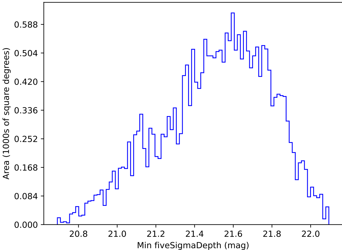
too_elab_r32_d3_gz_v3.4_10yrs Yr 1 y band: Min fiveSigmaDepth
