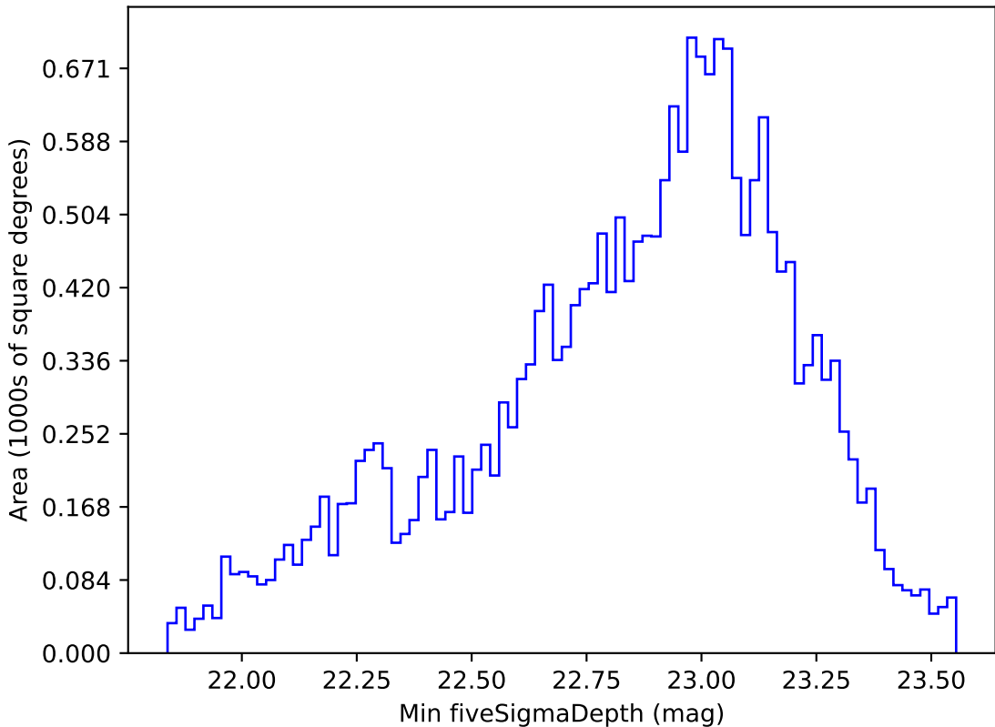
too_elab_r32_d3_gz_v3.4_10yrs Yr 1 u band: Min fiveSigmaDepth
