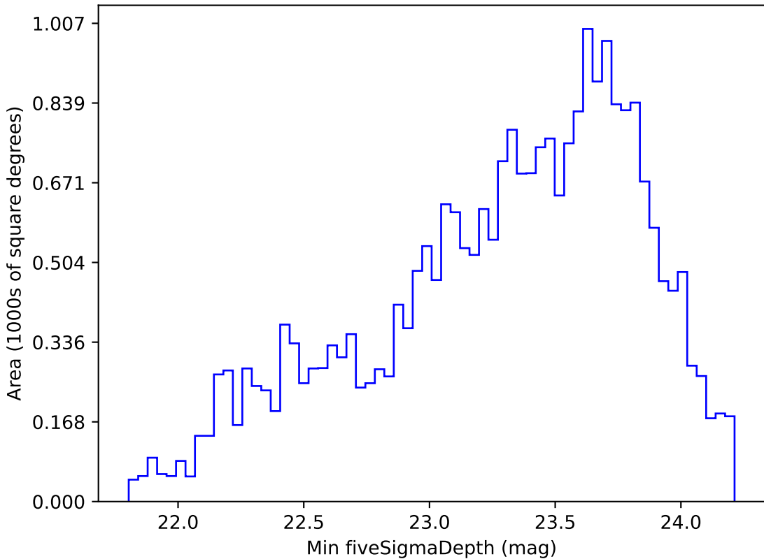
too_elab_r32_d3_gz_v3.4_10yrs Yr 1 r band: Min fiveSigmaDepth
