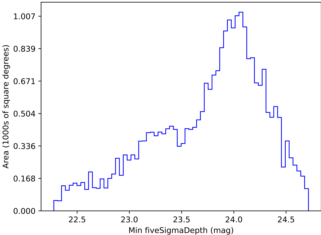
too_elab_r32_d3_gz_v3.4_10yrs Yr 1 g band: Min fiveSigmaDepth
