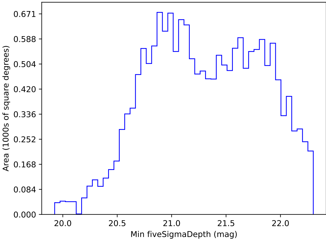
too_elab_r32_d3_gz_v3.4_10yrs WFD z band: Min fiveSigmaDepth
