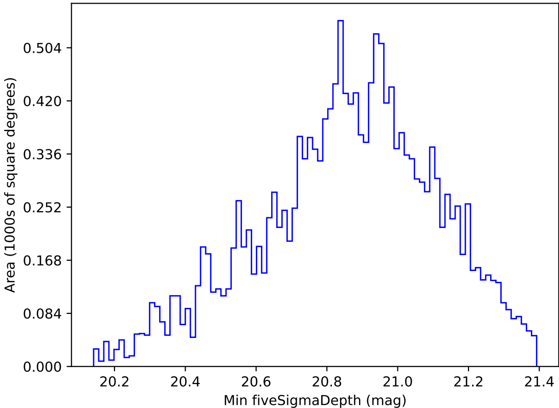
too_elab_r32_d3_gz_v3.4_10yrs WFD y band: Min fiveSigmaDepth
