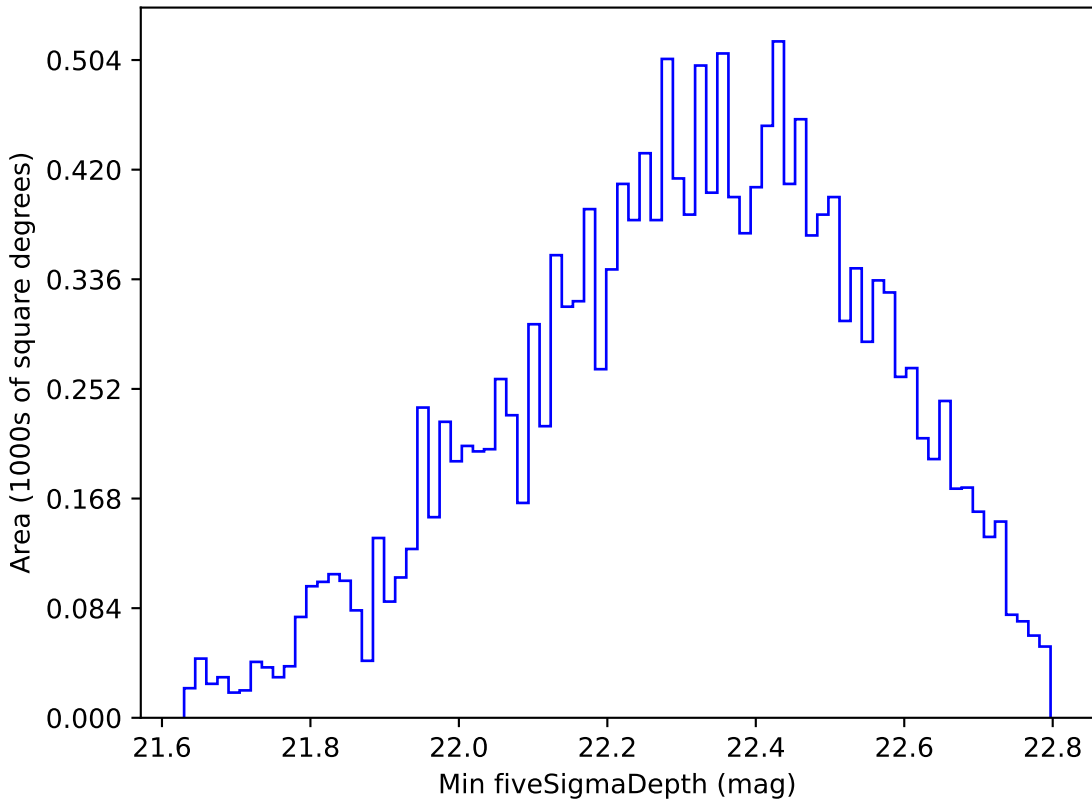
too_elab_r32_d3_gz_v3.4_10yrs WFD u band: Min fiveSigmaDepth
