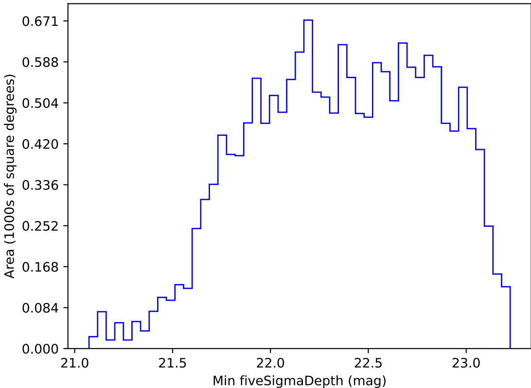
too_elab_r32_d3_gz_v3.4_10yrs WFD r band: Min fiveSigmaDepth
