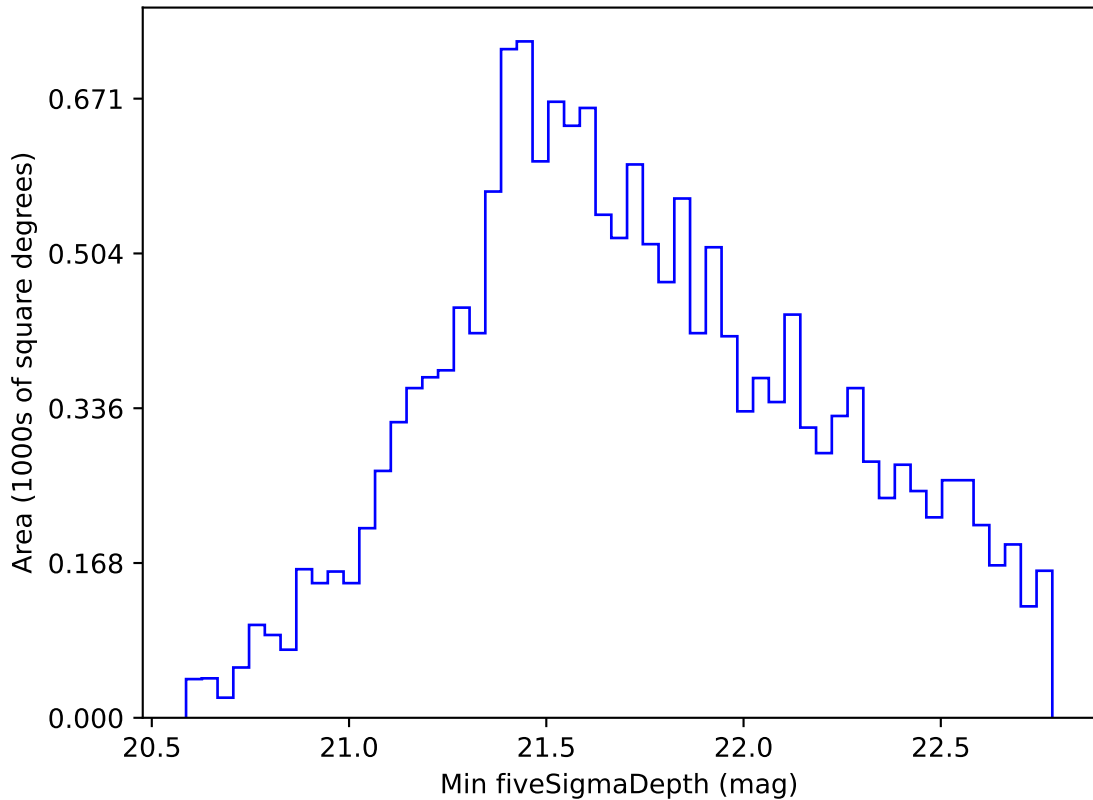
too_elab_r32_d3_gz_v3.4_10yrs WFD i band: Min fiveSigmaDepth
