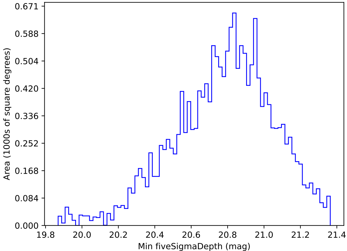
too_elab_r32_d3_gz_v3.4_10yrs WFD all bands: Min fiveSigmaDepth
