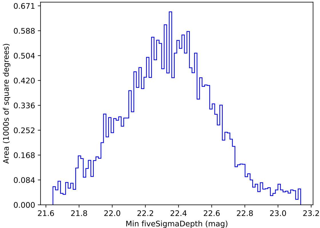
too_elab_r32_d3_gz_v3.4_10yrs All sky u band: Min fiveSigmaDepth
