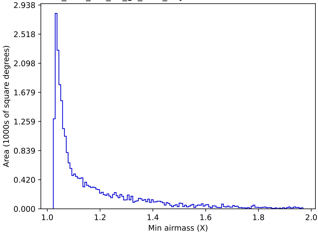
too_elab_r32_d3_gz_v3.4_10yrs Yr 1 z band: Min airmass
