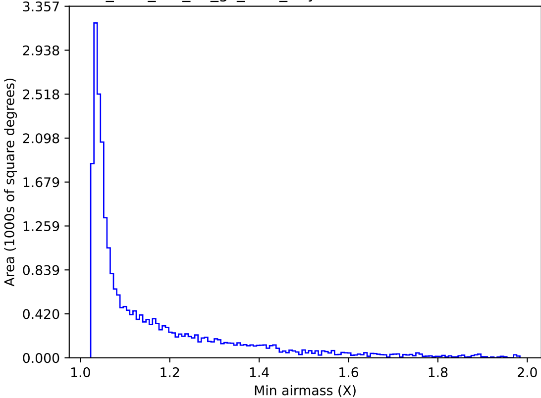
too_elab_r32_d3_gz_v3.4_10yrs Yr 1 r band: Min airmass
