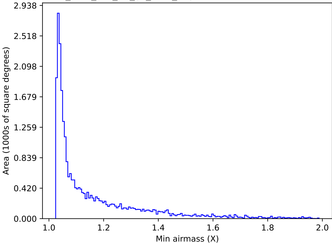
too_elab_r32_d3_gz_v3.4_10yrs Yr 1 i band: Min airmass
