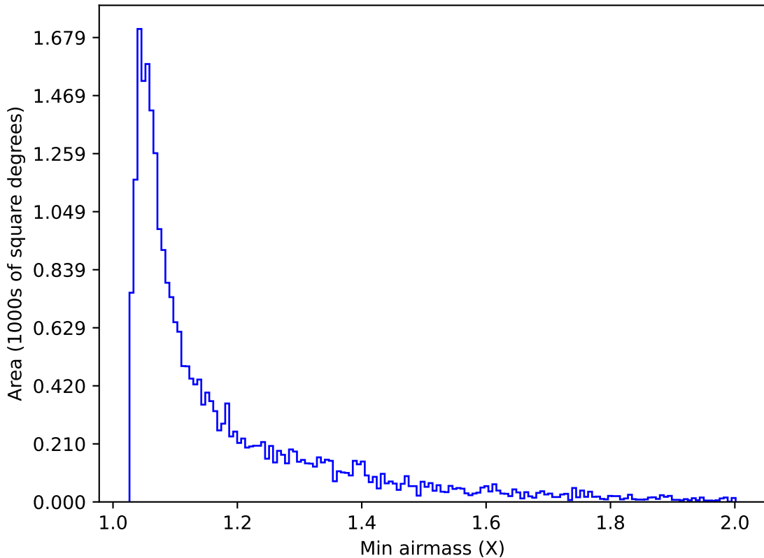
too_elab_r32_d3_gz_v3.4_10yrs Yr 1 g band: Min airmass
