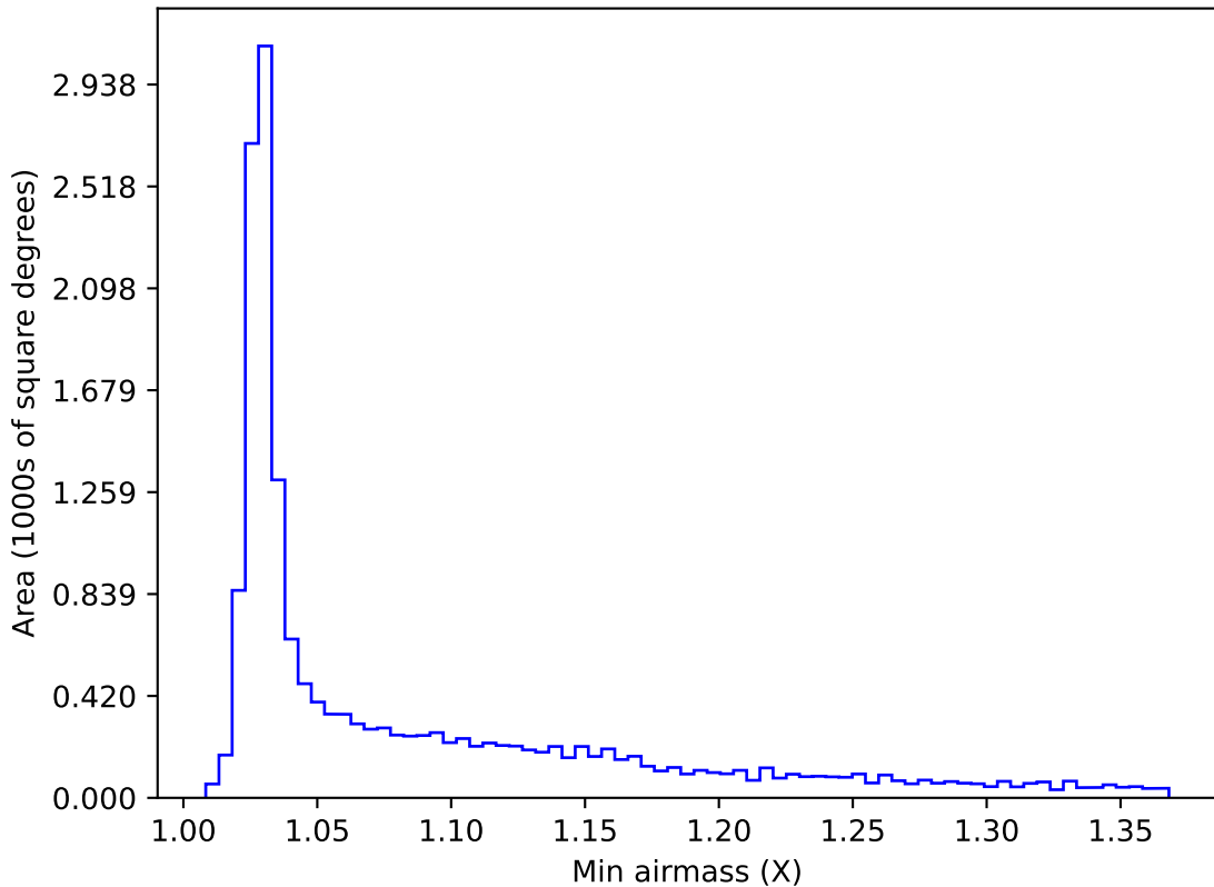
too_elab_r32_d3_gz_v3.4_10yrs WFD z band: Min airmass
