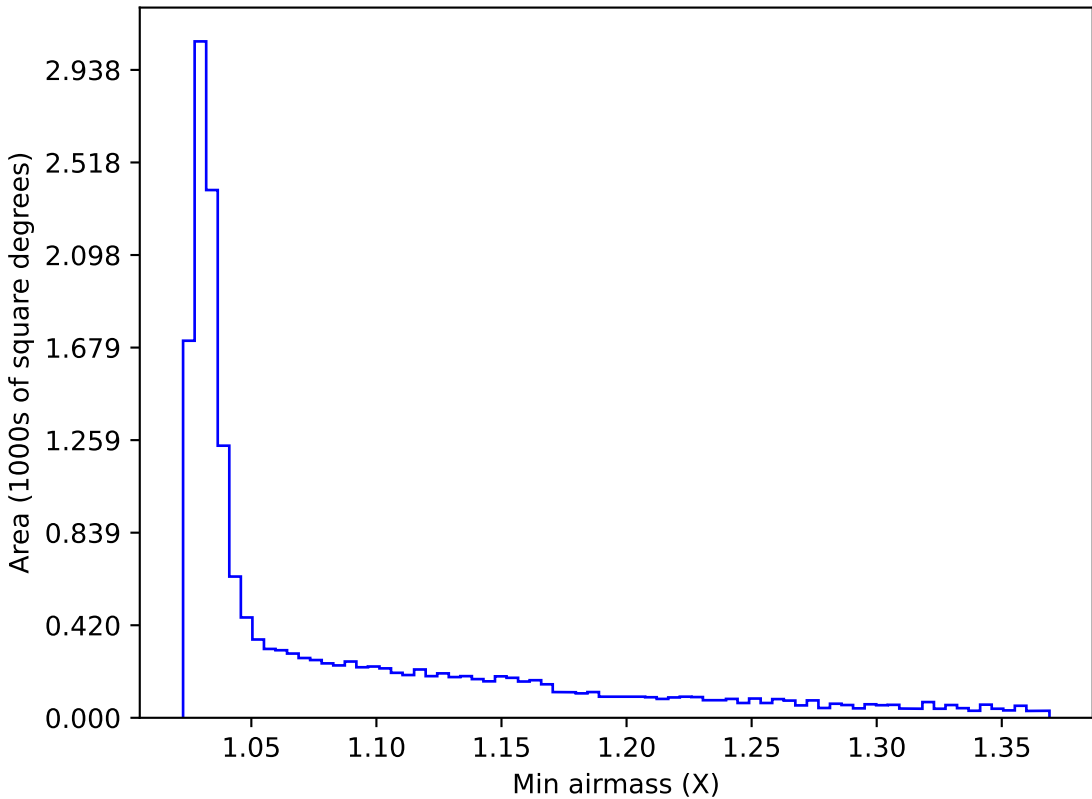
too_elab_r32_d3_gz_v3.4_10yrs WFD y band: Min airmass
