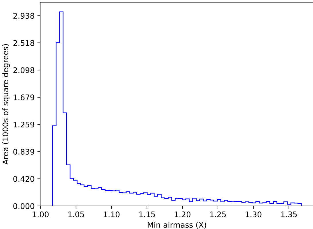
too_elab_r32_d3_gz_v3.4_10yrs WFD r band: Min airmass
