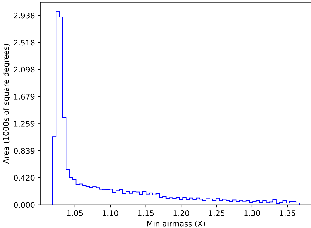
too_elab_r32_d3_gz_v3.4_10yrs WFD i band: Min airmass
