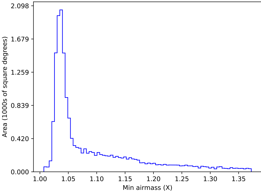
too_elab_r32_d3_gz_v3.4_10yrs WFD g band: Min airmass
