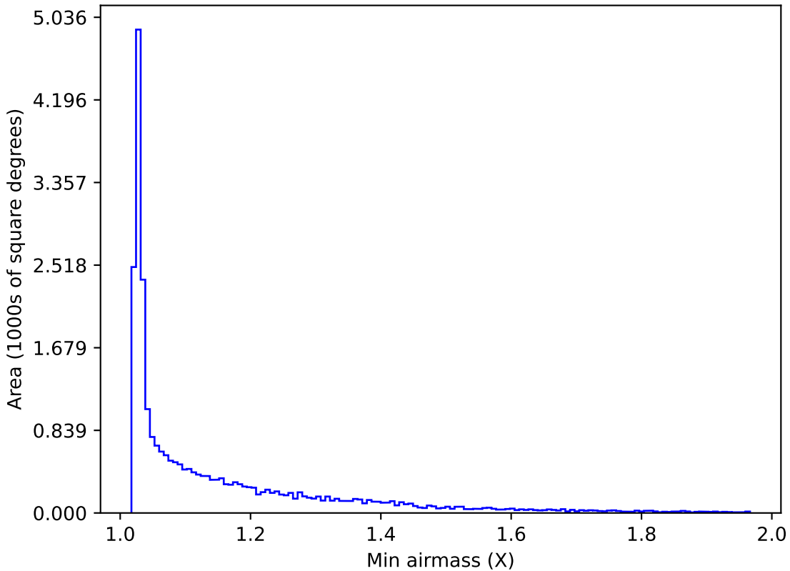
too_elab_r32_d3_gz_v3.4_10yrs All sky r band: Min airmass
