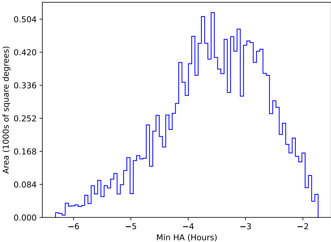
too_elab_r32_d3_gz_v3.4_10yrs WFD y band: Min HA
