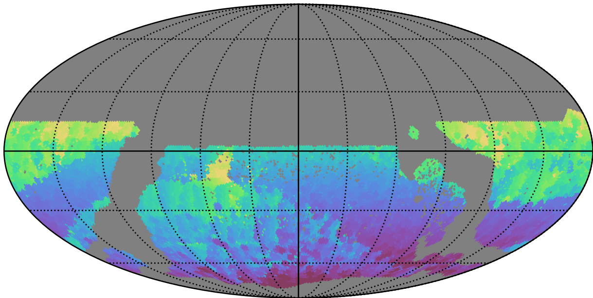
too_elab_r32_d3_gz_v3.4_10yrs WFD r band: Min HA
