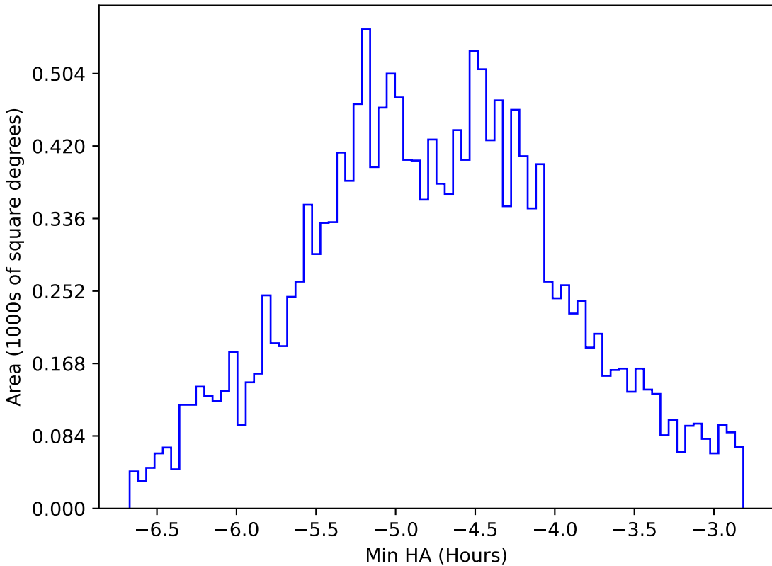
too_elab_r32_d3_gz_v3.4_10yrs WFD all bands: Min HA
