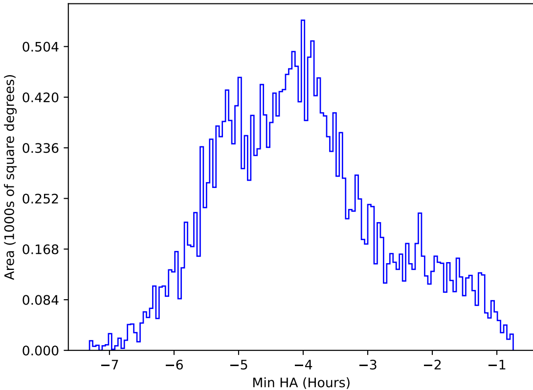
too_elab_r32_d3_gz_v3.4_10yrs All sky z band: Min HA
