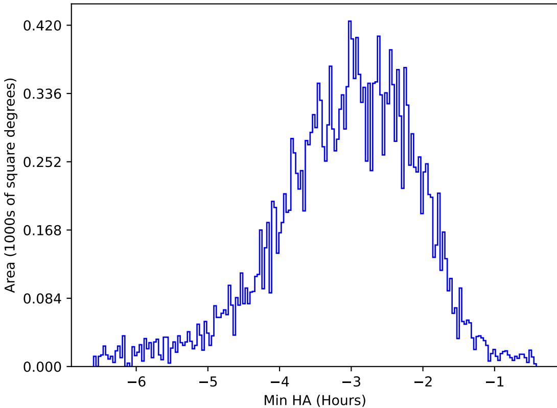
too_elab_r32_d3_gz_v3.4_10yrs All sky u band: Min HA
