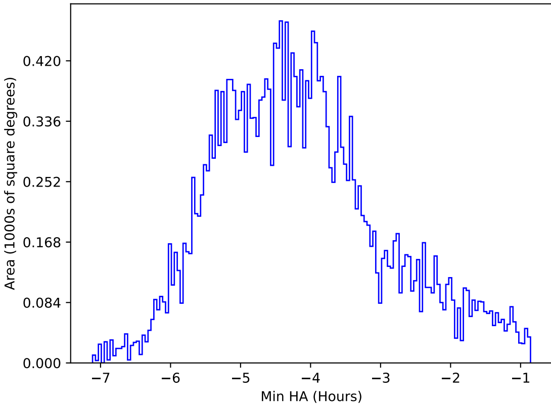
too_elab_r32_d3_gz_v3.4_10yrs All sky r band: Min HA
