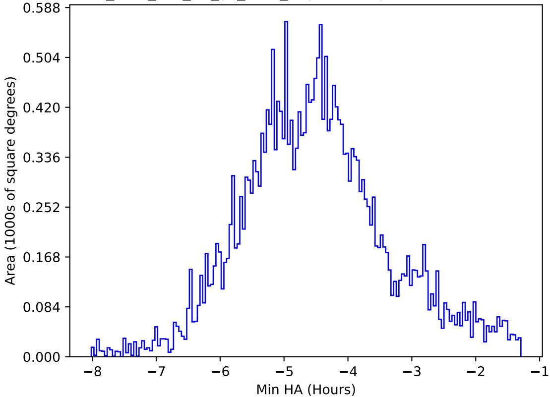
too_elab_r32_d3_gz_v3.4_10yrs All sky all bands: Min HA
