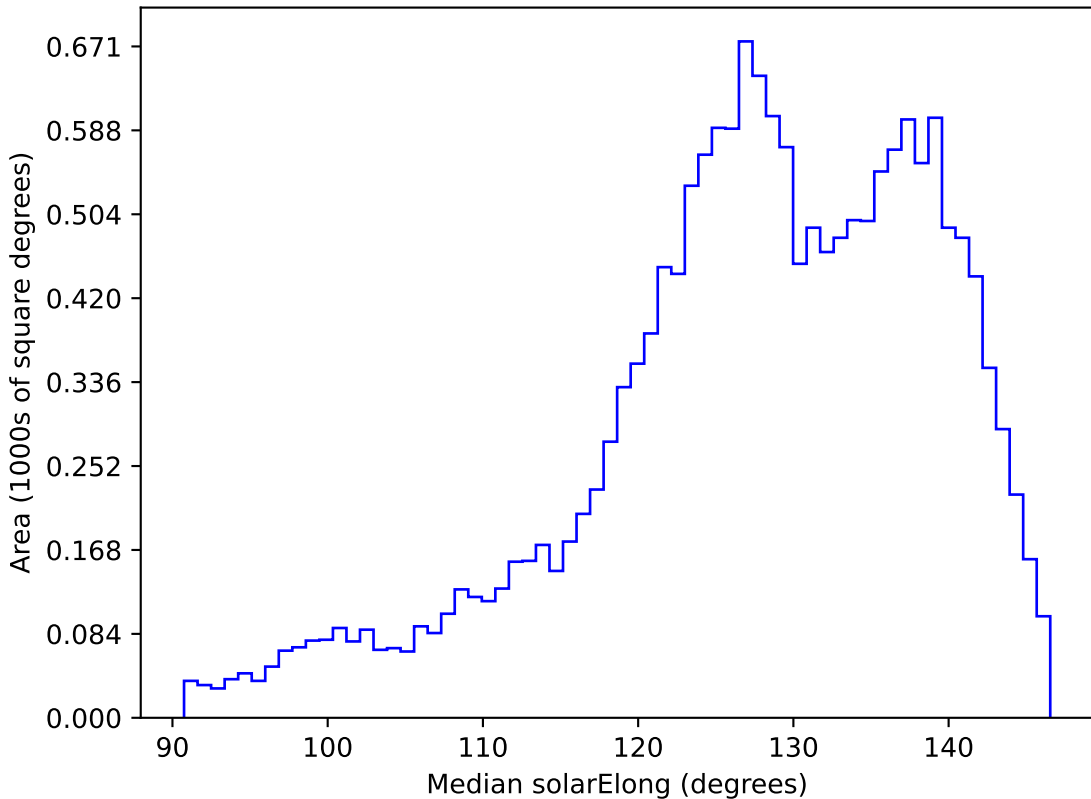
too_elab_r32_d3_gz_v3.4_10yrs WFD z band: Median solarElong
