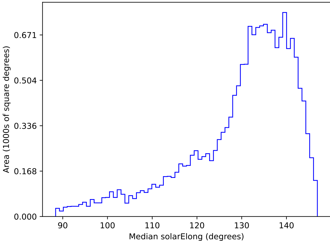
too_elab_r32_d3_gz_v3.4_10yrs WFD y band: Median solarElong
