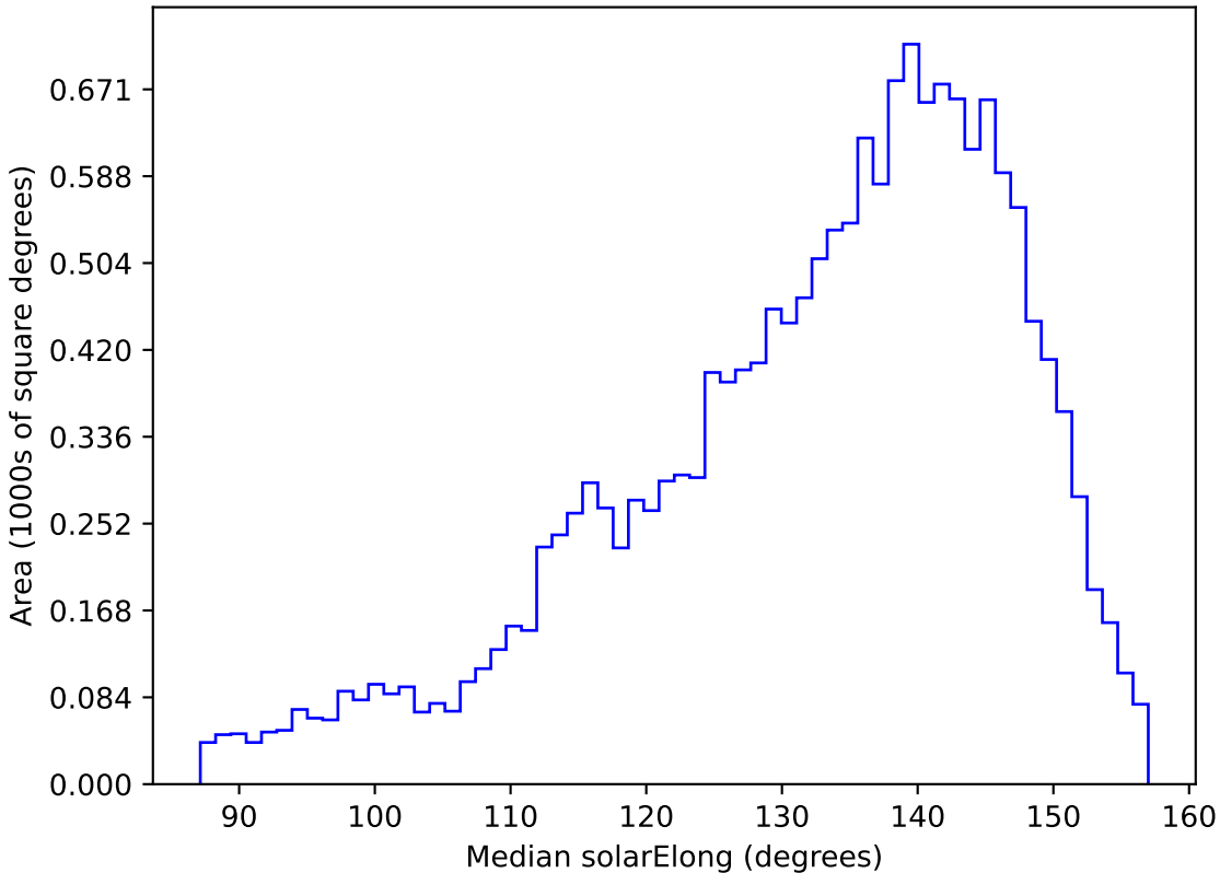
too_elab_r32_d3_gz_v3.4_10yrs WFD u band: Median solarElong
