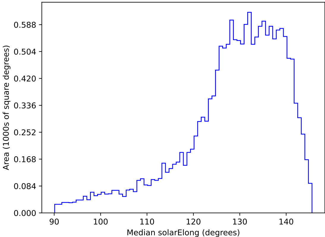
too_elab_r32_d3_gz_v3.4_10yrs WFD i band: Median solarElong
