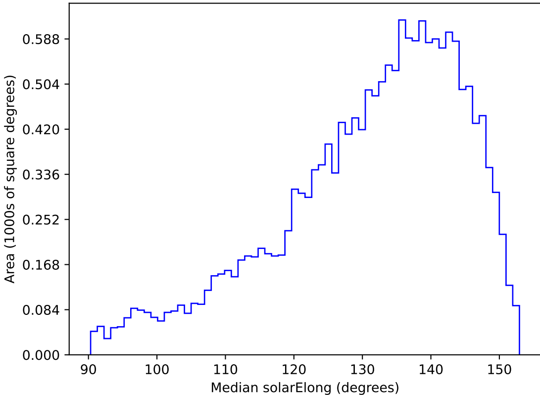
too_elab_r32_d3_gz_v3.4_10yrs WFD g band: Median solarElong
