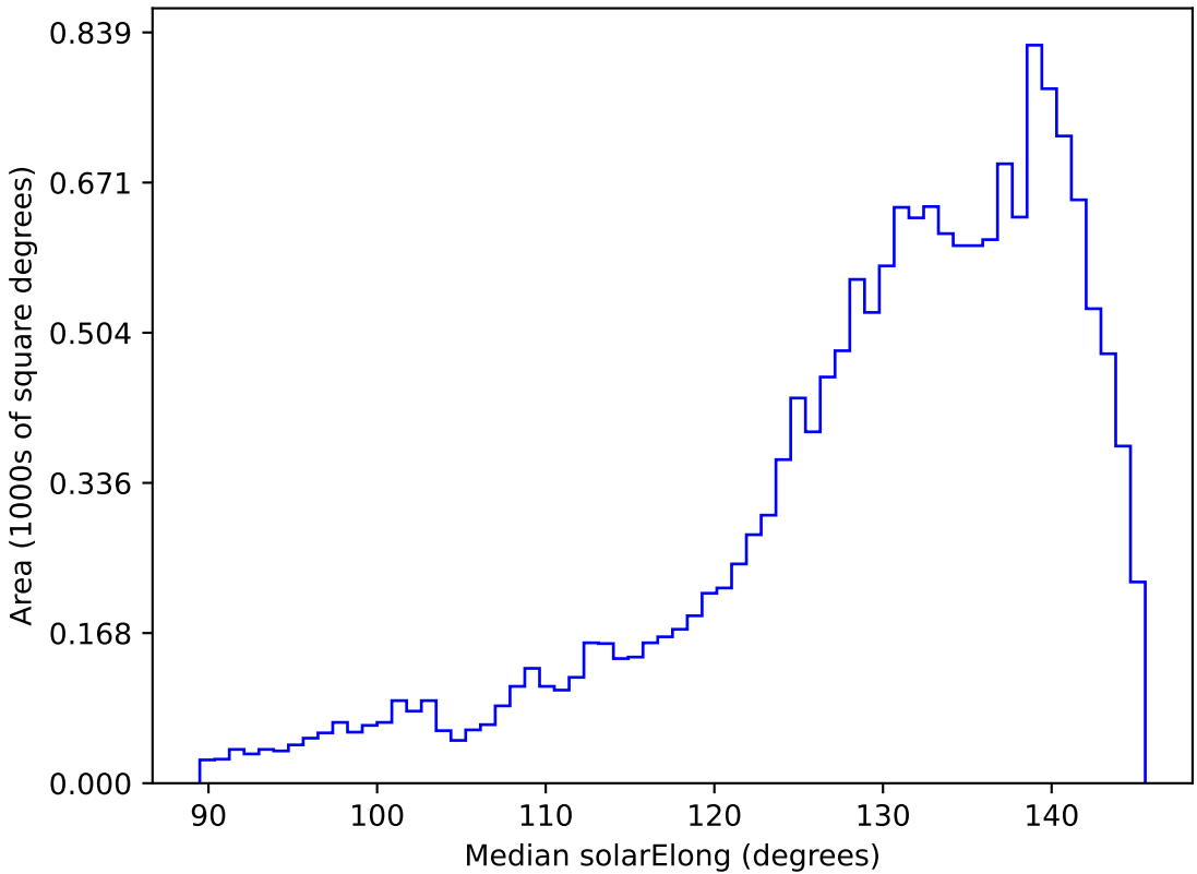
too_elab_r32_d3_gz_v3.4_10yrs WFD all bands: Median solarElong
