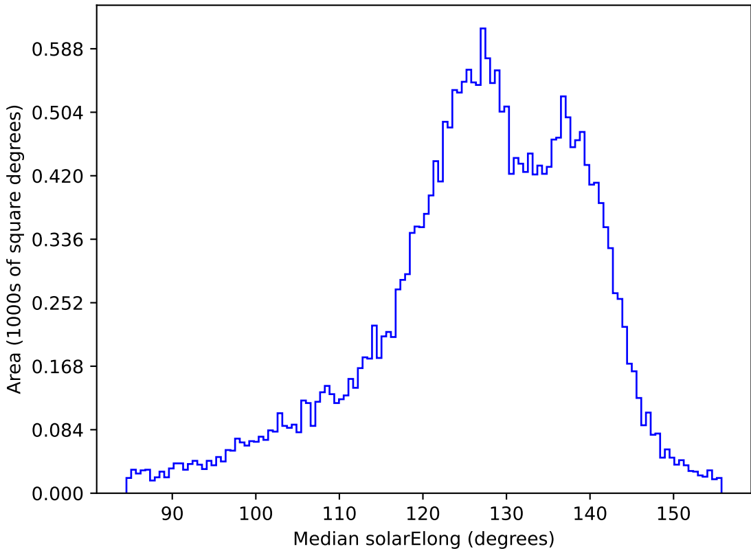
too_elab_r32_d3_gz_v3.4_10yrs All sky z band: Median solarElong
