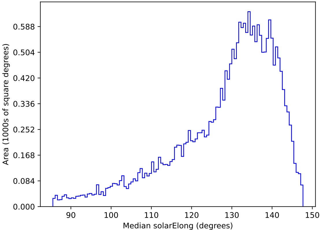
too_elab_r32_d3_gz_v3.4_10yrs All sky y band: Median solarElong
